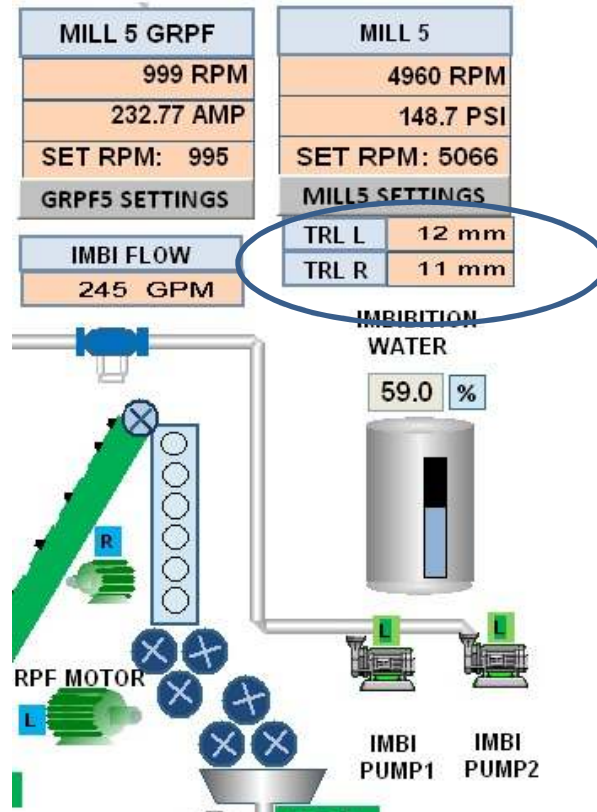
Actual Partial SCADA Screen Shot of Top Roller Lift Indication in Sugar Mill Automation and Control System
